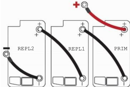
3 x 12V series (36V system)
